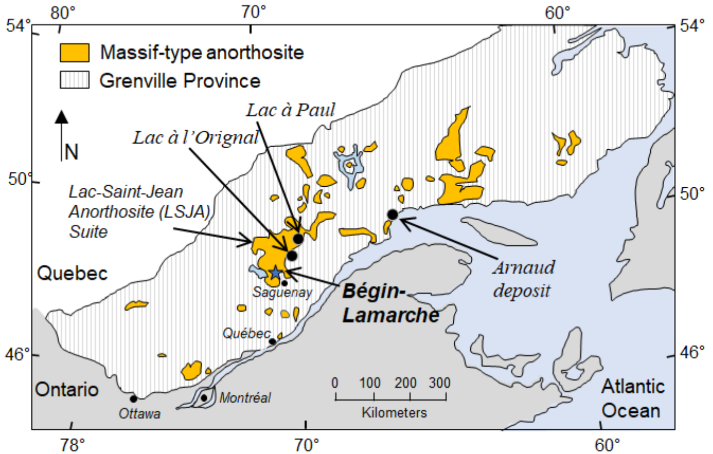
Fig. 2. Location map showing massif-type anorthosite bodies and the Bégin-Lamarche deposit, Quebec within the Grenville Province in Canada (modified after Banerjee et al., 2024b, Bédard, 2009; and Higgins et al., 2002). The three massif anorthosite-hosted phosphate deposits (Lac à l'Original, Arnaud, and Lac à Paul) evaluated for developing phosphate mines were also shown.
