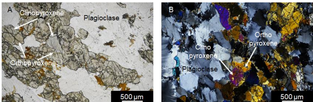
Fig. 14. Textural relationships of clinopyroxene from the Bégin-Lamarche deposit (under transmitted light). (A) Clinopyroxene crystals associated with orthopyroxene and plagioclase (sample LM18; plane-polarized light); (B) Clinopyroxene crystals associated with orthopyroxene and plagioclase (sample LM18; cross-polarized light).
