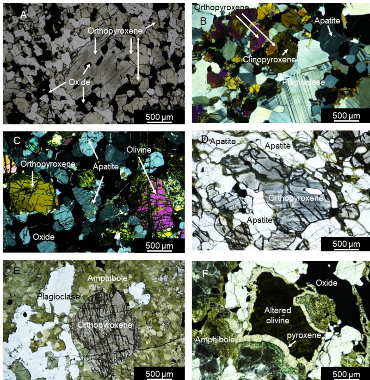
Fig. 11. Textural relationships of orthopyroxene from the Bégin-Lamarche deposit (under transmitted light). (A) Orthopyroxene crystals associated with oxide minerals (sample LM17; plane-polarized light); oxide minerals are also present as inclusions within orthopyroxene; (B) cumulate texture of orthopyroxene, clinopyroxene, and plagioclase (sample LM39; cross-polarized light); (C) Orthopyroxene crystals associated with olivine, apatite, and oxide minerals (sample LM25; cross-polarized light); (D) Orthopyroxene crystal surrounded by apatite crystals (sample LM6; plane-polarized light); (E) Orthopyroxene crystal surrounded by amphibole crystals (sample LM5; plane-polarized light) and (F) Corona structure where (ortho/clino) pyroxene forms a band around altered olivine and amphibole forms band around the pyroxene (sample LM31; plane-polarized light).
