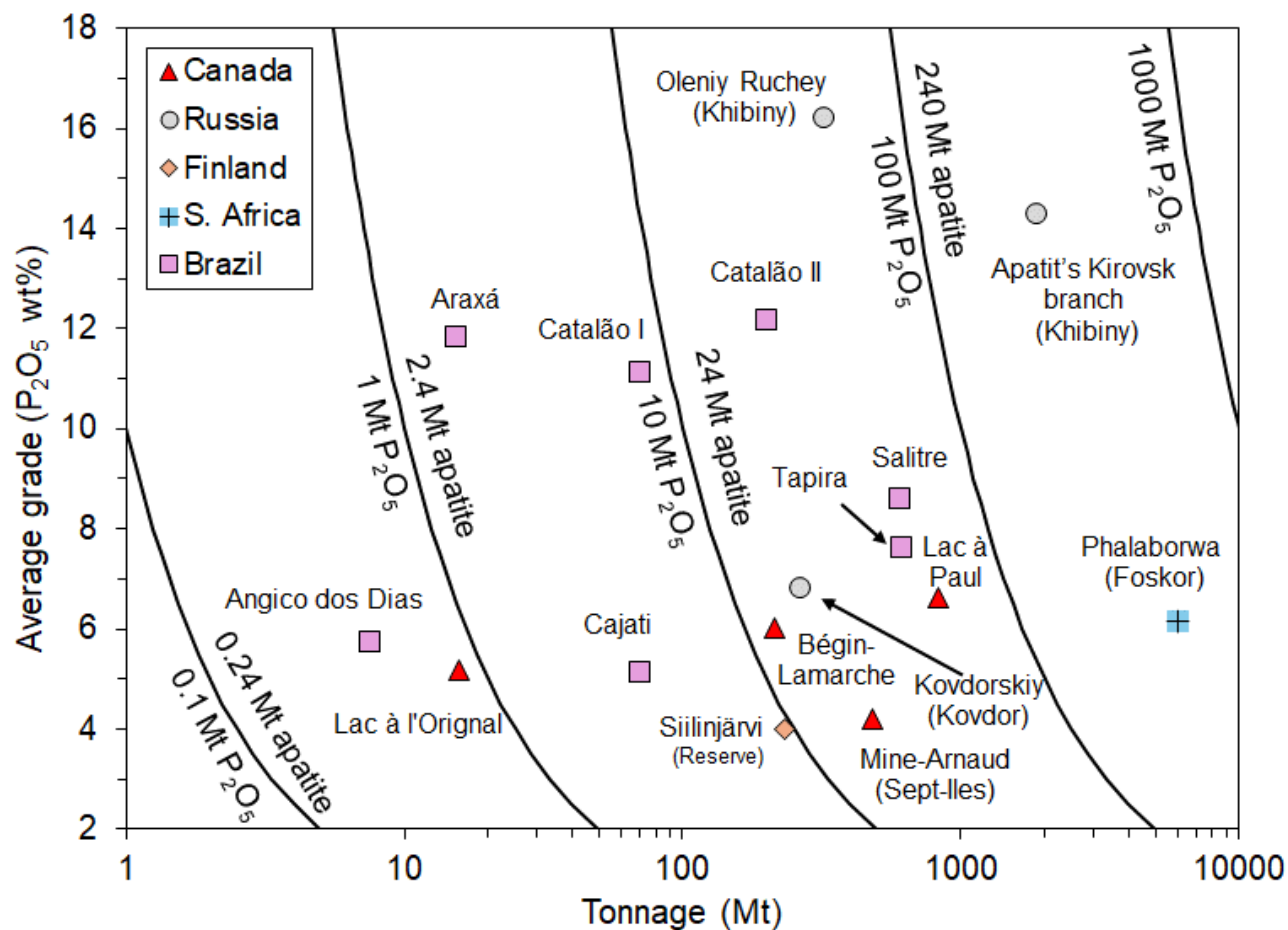
Fig. 3. Average grade versus tonnage (resource) for major igneous phosphate deposits from silica-undersaturated alkali and carbonatite intrusions from various countries around the world (modified after Banerjee et al., 2024a). The resources (tonnage) for Russian deposits (Oleniy Ruchey, Apatit's Kirovsk branch, and Kovdorskiy) are considered from the A+B+C1 reserve. Igneous phosphate deposits in Canada (prospective mines) hosted in oxide-apatite-mafic-ultramafic rocks within massif-anorthosites are also shown. Note that the tonnage (x)-axis is on a logarithmic scale. The curvilinear lines indicate the amount (Mt.) of P 2 O 5 or apatite within the phosphate ore.
