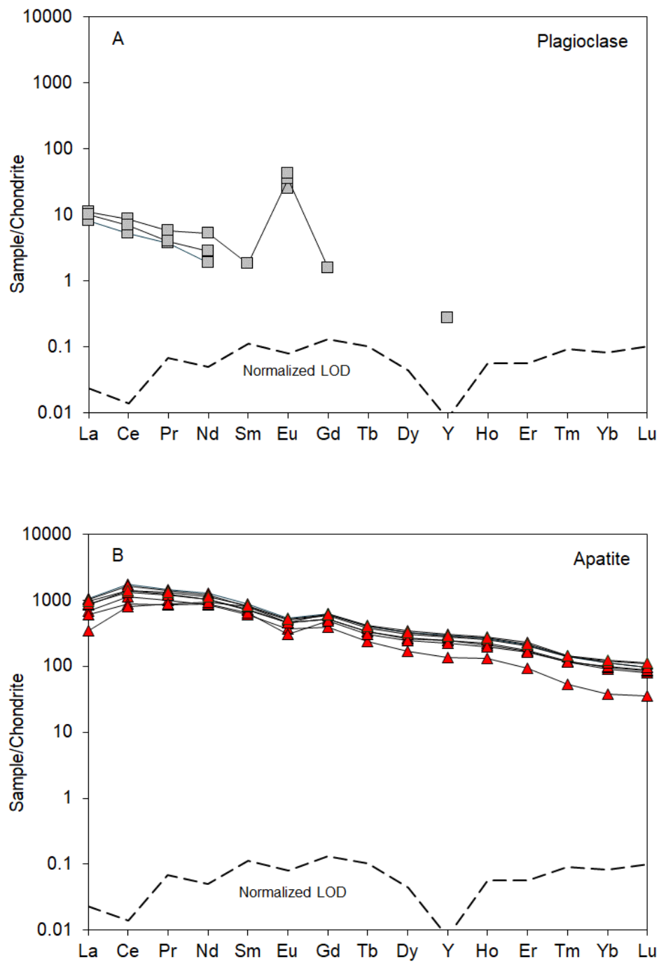
Fig. 30. Chondrite-normalized REE patterns of (A) plagioclase and (B) apatite crystals from the Bégin-Lamarche deposit (North and South Zone).
