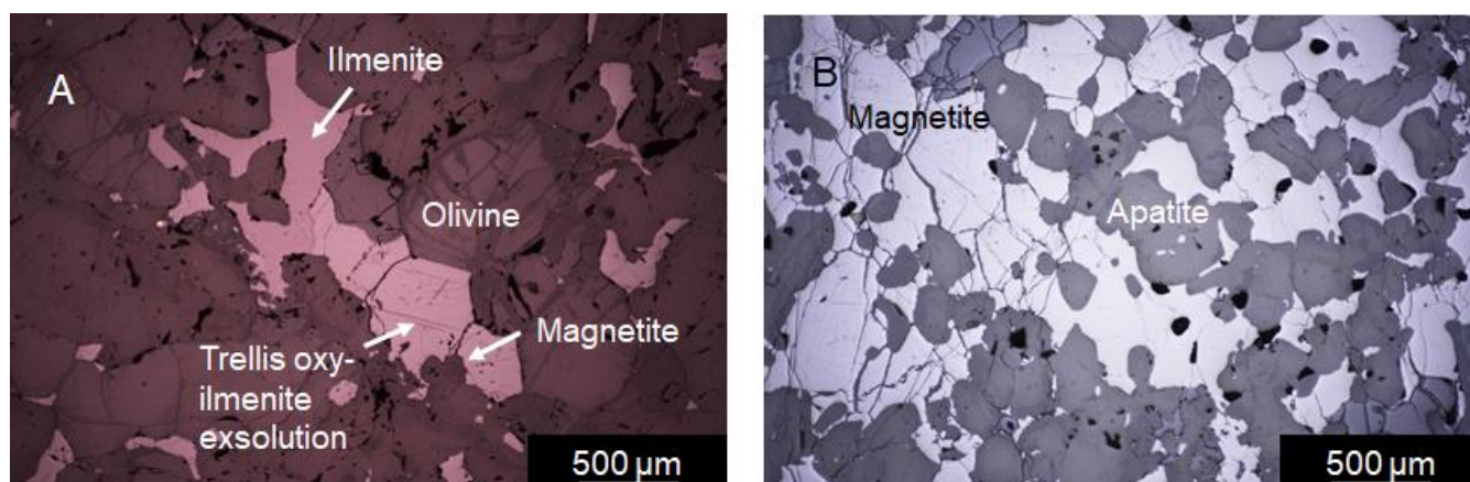
Fig. 27. Textural relationships of magnetite from the Bégin-Lamarche deposit (under reflected light). (A) Magnetite and ilmenite crystals associated with olivine crystals (sample LM8); note the presence of trellis oxy-ilmenite exsolution in magnetite; (B) Magnetite crystals associated with apatite crystals (sample LM36).
