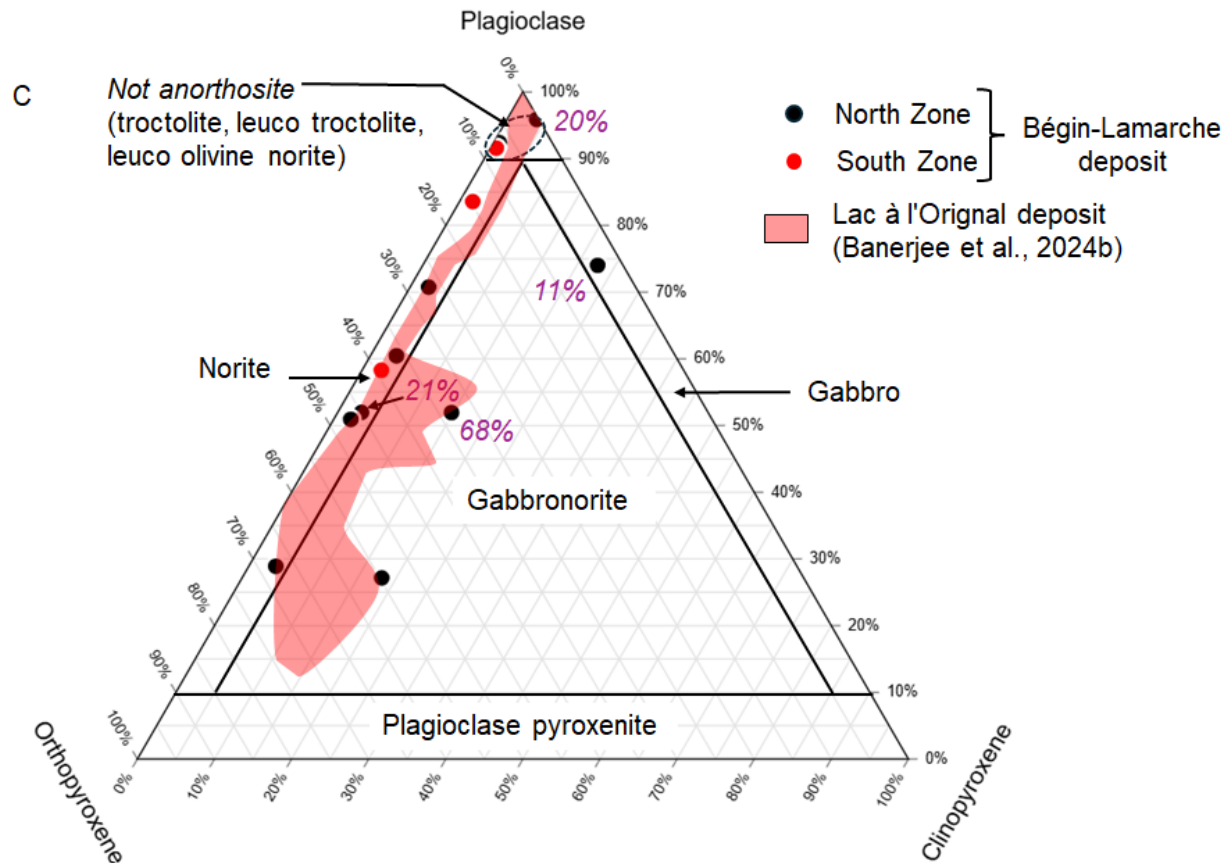
Fig. 8. Comparisons of anorthosite hosted oxide-apatite mafic and ultramafic rock types of three phosphate deposits (Bégin-Lamarche, Lac à l'Original, and Lac à Paul) in Quebec. Anorthosite and plagioclase-bearing ultramafic rocks from the Bégin-Lamarche deposit were not included in Figure C. High abundances (11-68 %) of amphibole for the four samples of the Bégin-Lamarche are also reported (in % values; in italic ) in Figure C. Abbreviations: magnetite, mt; ilmenite, ilm; Al-spinel, Al-spi.
