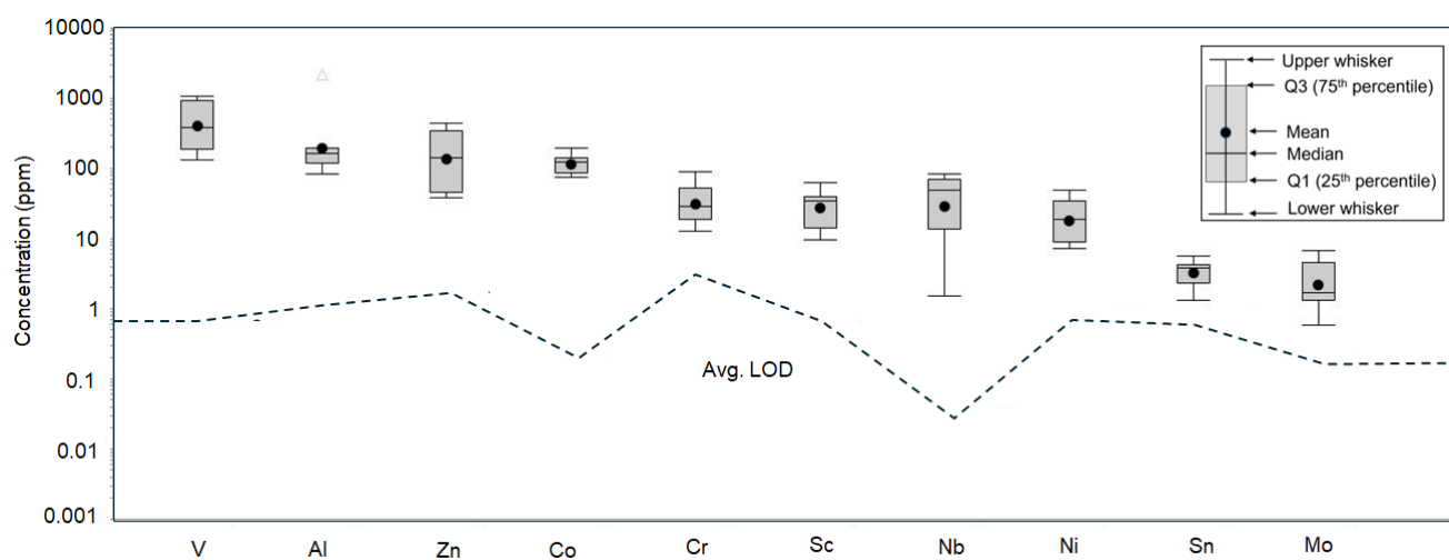
Fig. 26. Concentrations of selected trace elements in ilmenite (n=9 samples) of the Bégin-Lamarche deposit (North and South Zone). The less than LOD values (<LOD) are replaced by LOD/2. The elements are arranged by their decreasing concentrations.
