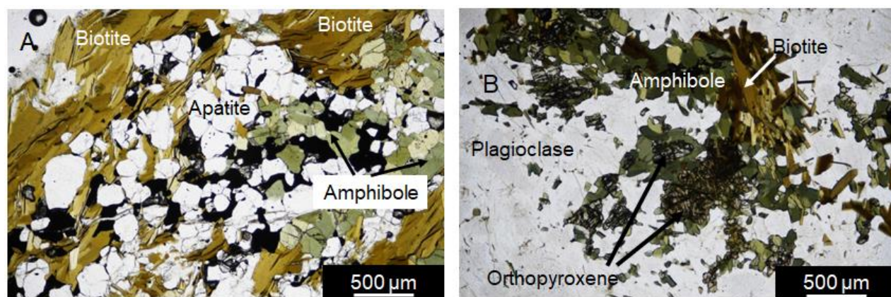
Fig. 18. Textural relationships of biotite from the Bégin-Lamarche deposit (under transmitted plane-polarized light). (A) Biotite crystals associated with apatite and amphibole crystals (sample LM16); (B) Biotite crystals associated with amphibole and plagioclase crystals (sample LM2); Note the orthopyroxene surrounded by amphibole.
