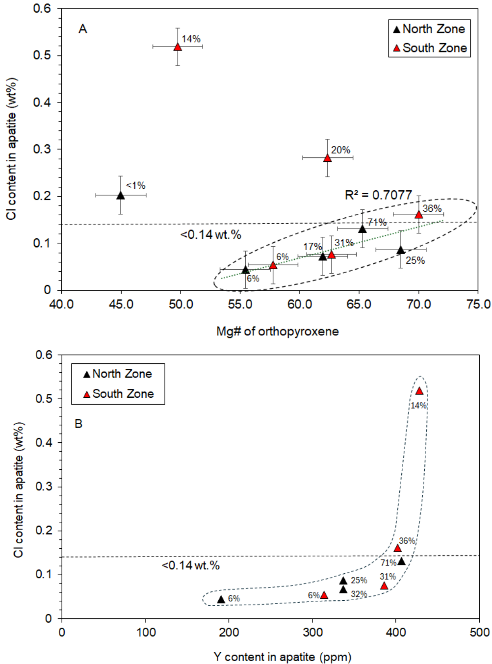
Fig. 23. (A) Relationships between Cl contents of apatite (fluorapatite) and Mg# of coexisting orthopyroxene from the rocks of the Bégin-Lamarche deposit (North and South Zone); (B) Relationships between Cl and Y contents in apatite from the rocks of the Bégin-Lamarche deposit. Apatite abundances (in % values) are shown in Figures. The upper limits of the Cl content of saleable phosphate ore (<0.14 wt.%) suggested by Yara International are also shown (Païement et al., 2013). The average standard deviations of data (bar and whiskers) are also shown in Figure A, as calculated using \text{avg. SD} = \sqrt{(S_1^2 + S_2^2 + \dots + S_k^2)/k} ; where S_k = standard deviation for the 'k'th sample and k = total number of samples (Cohen, 1988).
