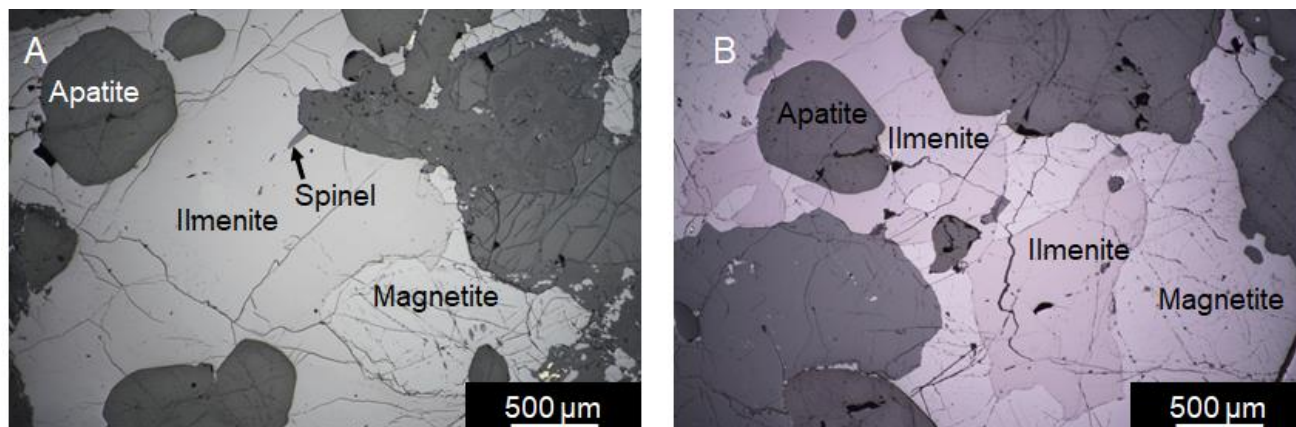
Fig. 25. Textural relationships of ilmenite from the Bégin-Lamarche deposit (under reflected light). A (sample LM 23) and B (sample LM28) showing ilmenite crystals associated with magnetite and apatite crystals.
