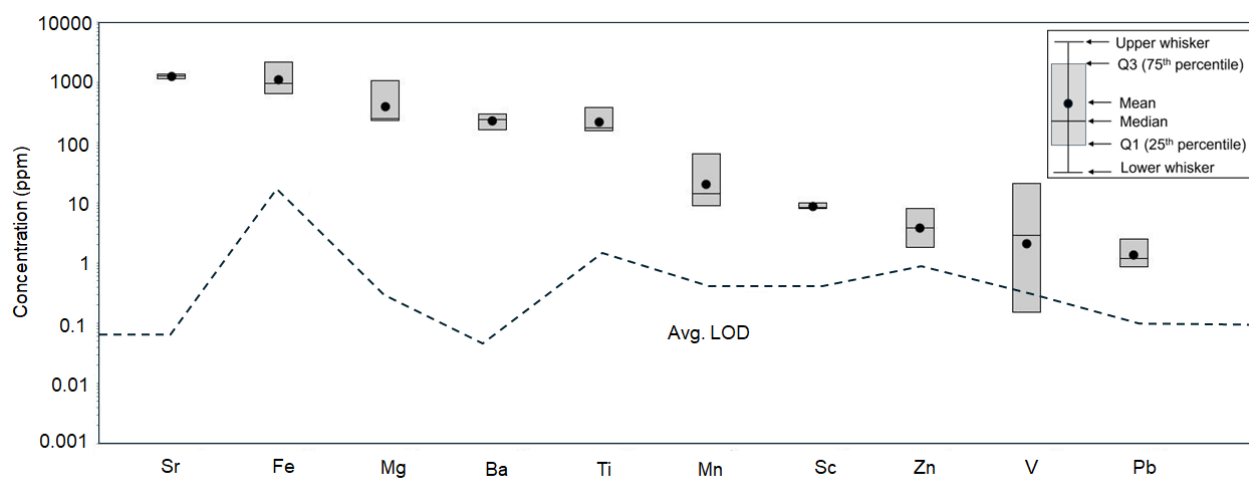
Fig. 16. Concentrations of selected trace (and minor) elements in plagioclase (n=3 samples) of the Bégin-Lamarche deposit (North and South Zone). The less than LOD values (<LOD) are replaced by LOD/2. The elements are arranged by their decreasing concentrations.
