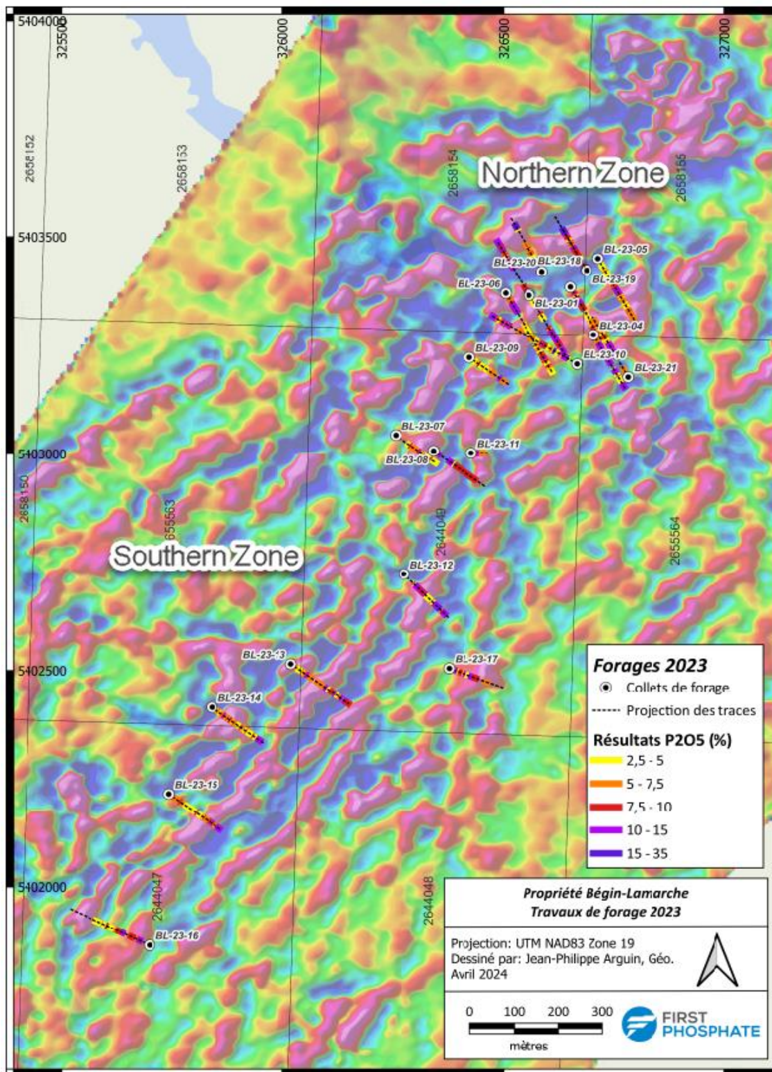
Fig. 5. Drill hole distributions within the North and South Zone of the Bégin-Lamarche property of First Phosphate Corp.
