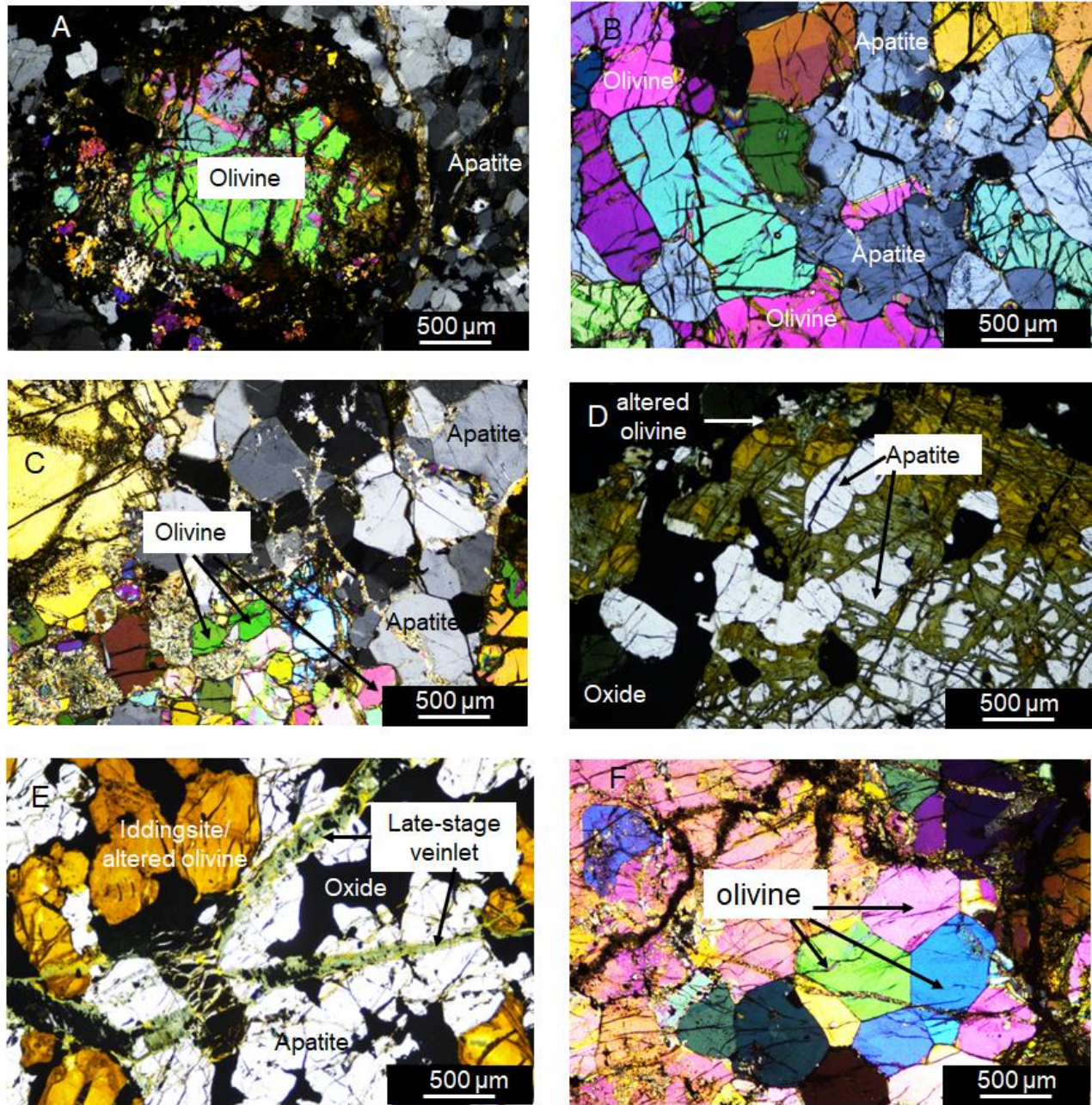
Fig. 9. Textural relationships of olivine from the Bégin-Lamarche deposit (under transmitted light). (A) Fractured olivine crystal surrounded by apatite (sample LM1; cross-polarized light); (B) Cumulate texture of olivine and apatite (sample LM12; cross-polarized light); (C) Small size crystals of olivine associated with larger size apatite crystals (sample LM8; cross-polarized light); (D) Altered olivine associated with apatite and oxide minerals (sample LM4; plane-polarized light); (E) Iddingsite (altered olivine) associated with apatite and oxide minerals; late-stage veinlets cross cut iddingsite and apatite (sample LM4; plane-polarized light); (F) Olivine crystals with straight triple junction crystal boundaries (LM8; cross-polarized light).
