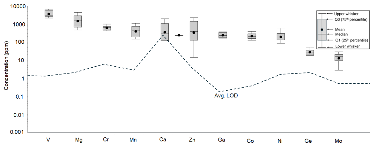
Fig. 28. Concentrations of selected trace (and minor) elements in magnetite (n=8 samples) of the Bégin-Lamarche deposit (North and South Zone). The less than LOD values (<LOD) are replaced by LOD/2. The elements are arranged by their decreasing concentrations.
