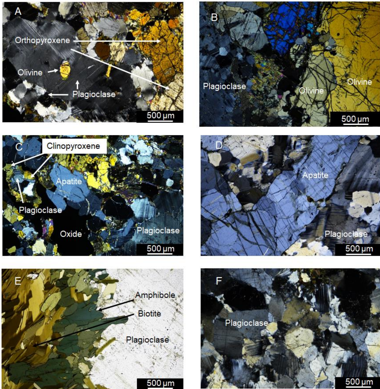
Fig. 15. Textural relationships of plagioclase from the Bégin-Lamarche deposit (under transmitted light). (A) Cumulate texture of orthopyroxene and plagioclase; olivine is also present as inclusion within a plagioclase crystal (sample LM15; cross-polarized light); (B) Plagioclase crystals associated with olivine crystals (sample LM7; cross-polarized light); (C) Different sizes of plagioclase crystals associated with clinopyroxene, apatite, and oxide minerals (sample LM21; cross-polarized light); (D) Plagioclase crystals associated with apatite crystals (sample LM48; cross-polarized light); (E) Plagioclase crystals associated with amphibole and biotite crystals (sample LM16; plane-polarized light); (F) Granoblastic texture of plagioclase crystals with serrated crystal boundaries in anorthosite (sample LM33; cross-polarized light).
