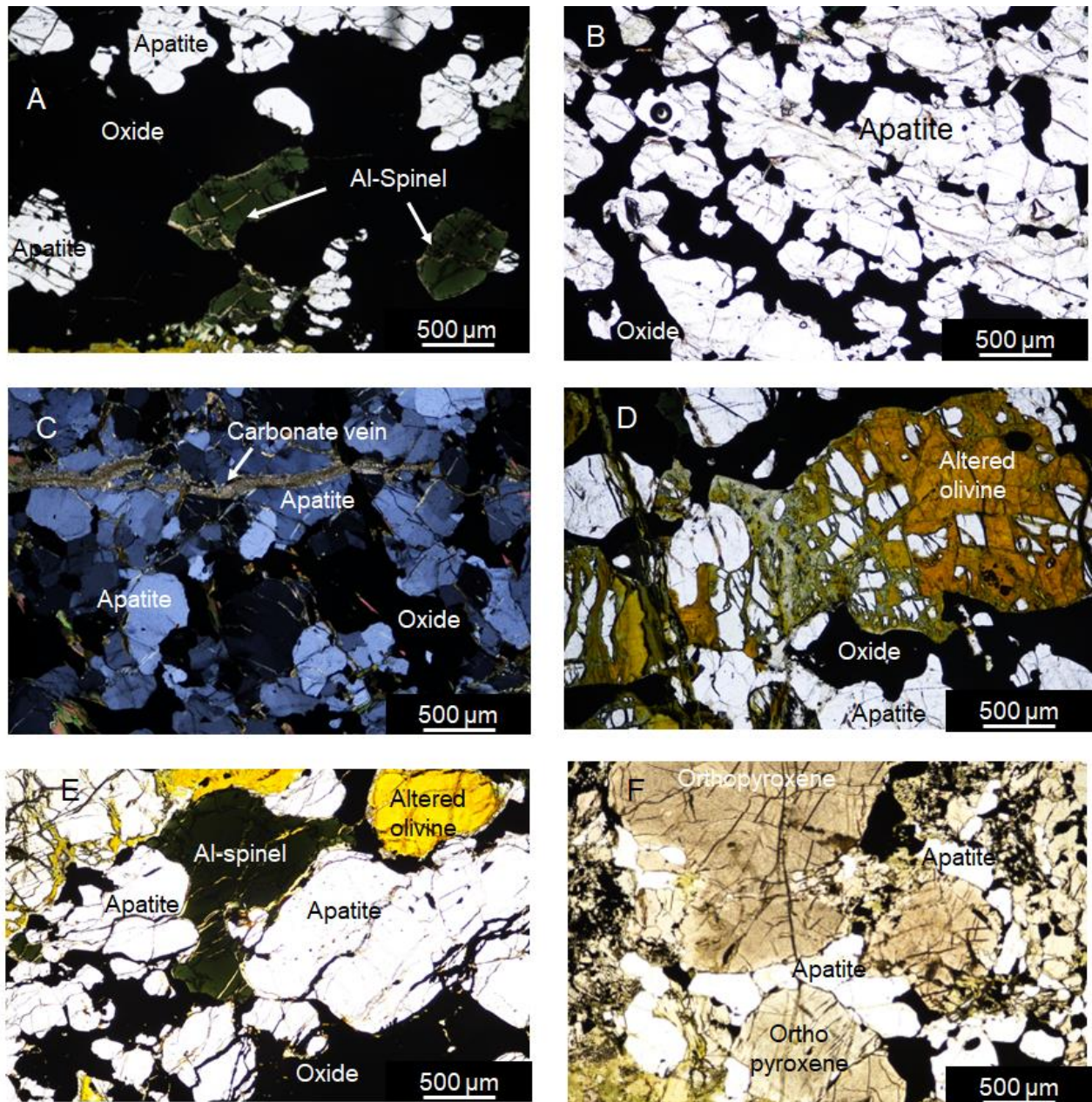
Fig. 19. Textural relationships of apatite from the Bégin-Lamarche deposit (under transmitted light). (A) Apatite crystals associated with oxide minerals and Al-spinel (sample LM4; plane-polarized light); (B) Apatite crystals with different sizes within oxide minerals-rich layer (sample LM49; plane-polarized light); (C) Apatite crystals associated with oxide minerals; a carbonate vein cross-cut apatite (sample LM44; cross-polarized light); (D) Apatite crystals associated with altered olivine (iddingsite) and oxide minerals (sample LM12; plane-polarized light); (E) Apatite crystals associated with altered olivine, Al-spinel, and oxide minerals (sample LM3; plane-polarized light); (F) Apatite crystals associated with orthopyroxene crystals (sample LM15; plane-polarized light).
