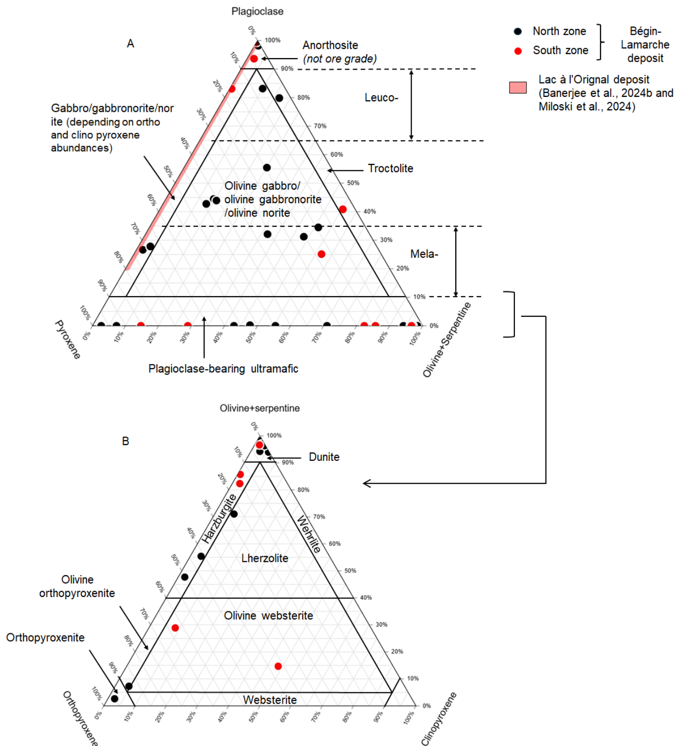
Fig. 7. Classification of oxide-apatite-mafic and ultramafic rocks of the Bégin-Lamarche deposit (North and South Zone). The distributions of plagioclase, pyroxene, and olivine+serpentine of the Lac à l'Original deposit are also shown in Fig. A
