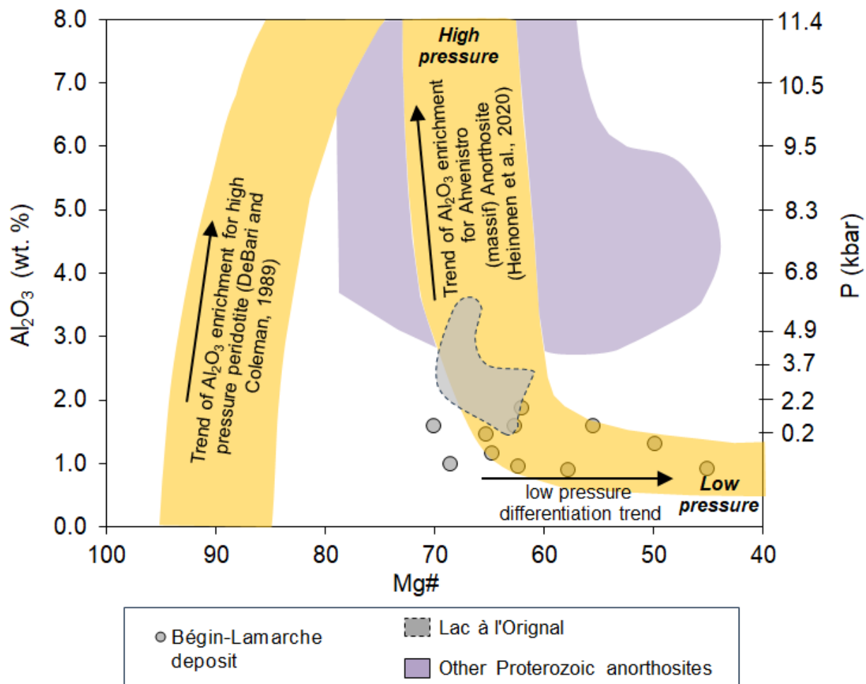
Fig. 12. Relationships between \text{Al}_2\text{O}_3 content and Mg# of orthopyroxene in the oxide-apatite-mafic-ultramafic rocks of the Bégin-Lamarche deposit (North and South Zone). Orthopyroxene from the Lac à l'Original deposit (Banerjee et al., 2024b; Miloski et al., 2024; Grant, 2020) and other Proterozoic anorthosites (Mealy Mountains Intrusive Suite, Nain Plutonic Suite, Canada; Bybee et al., 2014; Rogaland Anorthosite Province, Norway, Bybee et al., 2014; Charlier et al., 2010) are also shown. The Mg# of orthopyroxene from Miloski et al. (2024) and Grant (2020) are calculated from their \text{FeO}_{\text{total}} and MgO data of orthopyroxene. The pressures of orthopyroxene crystallization were calculated using the Al content of orthopyroxene from the Ahvenisto Anorthosite, Finland (Heinonen et al., 2020) according to the geobarometric relationship of Emslie et al. (1994).
