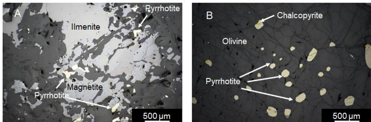
Fig. 29. Textural relationships of sulfide minerals from the Bégin-Lamarche deposit (under reflected light). (A) Pyrrhotite mineral associated with ilmenite and magnetite crystals (sample LM20); (B) Pyrrhotite crystals within olivine crystals (sample LM4).
