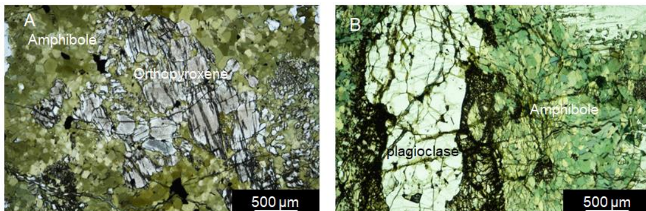
Fig. 17. Textural relationships of amphibole from the Bégin-Lamarche deposit (under transmitted plane-polarized light). (A) Amphibole crystals surrounding orthopyroxene crystal; note the conversion of orthopyroxene to amphibole (sample LM5); (B) Amphibole crystals associated with plagioclase crystals (sample LM40).
