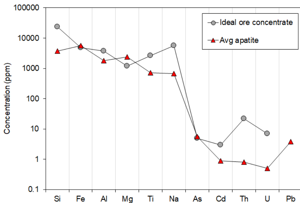
Fig. 31. Comparisons of selected elemental concentrations of ideal phosphate ore concentrate for phosphoric acid production (provided by Prayon), and average apatite crystals of the Bégin-Lamarche deposit (North and South Zone). Si, Fe, Al, Mg, Ti, and Na data of average apatite (Avg apatite) are from apatite concentrate (prepared and analyzed by SGS Canada), and As, Cd, Th, U, and Pb data of average apatite are from in-situ analysis of apatite crystals (analyzed in this study).
